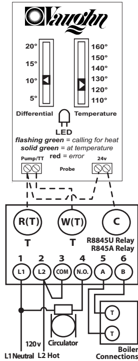
Switching Relay R8845U, R845A and SR 501
